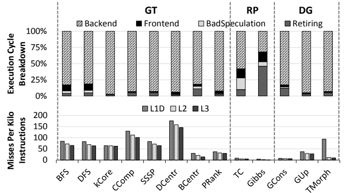
Fig. 2: Architectural behaviors of graph workloads on an Intel Xeon E5 machine
