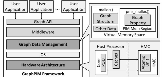
Fig. 5: Overview of GraphPIM framework
